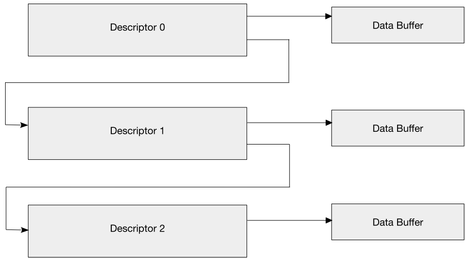
Figure 9-7. Descriptor Chain
