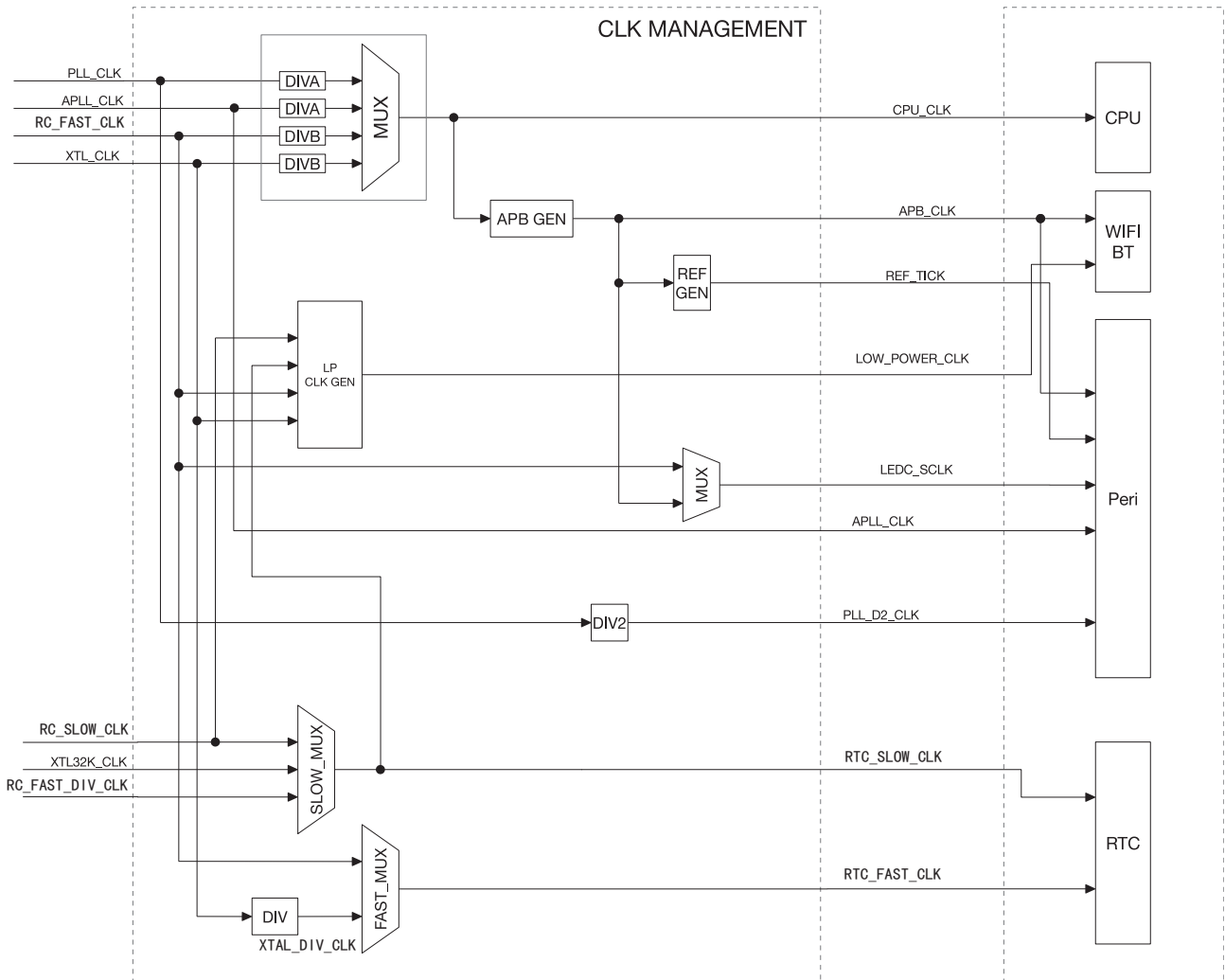
Figure 3-2. System Clock
