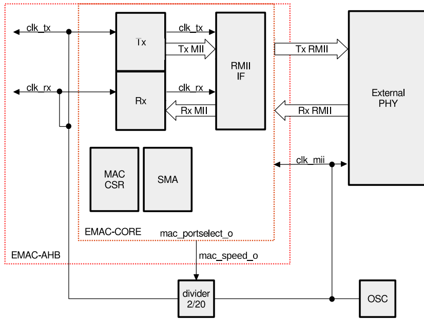
Figure 10-6. RMIIClock
